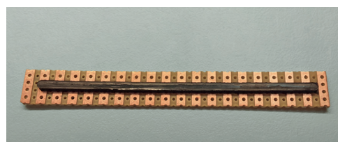
Test sample for the measurement of contact resistances of strand of electrically conductive composite on a circuit board
